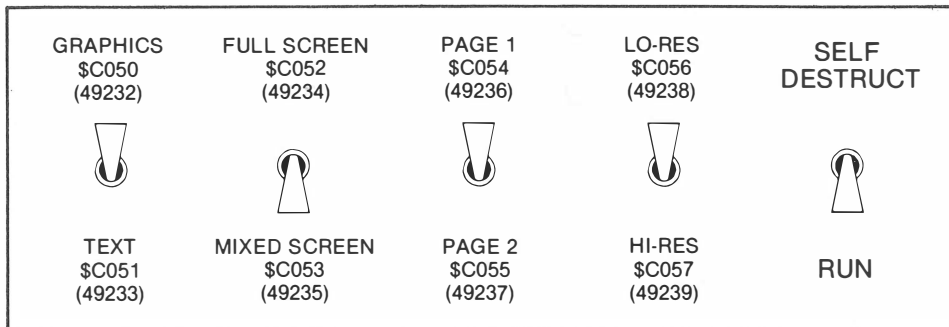
Figure 5-1. Toggle switches.
